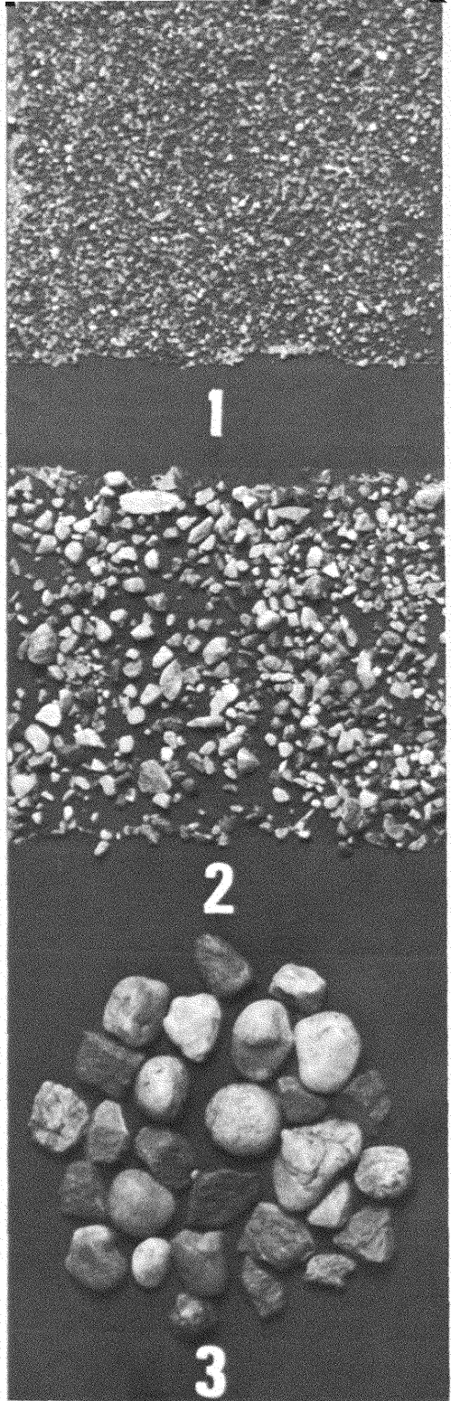
Figure 2: 1. Sand considered ideal for use in the top mixture (layer E in Figure 1). This is classified as a coarse to medium sand.
