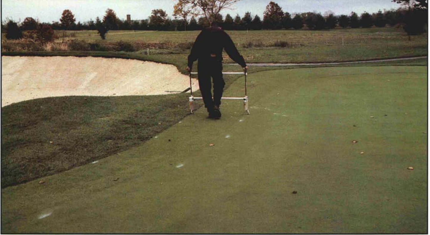
(Above) Originally two paint guns were used to mark the collar width of each green. The tool is held together with PVC pipe, but moves easily along flowing putting green contours.
